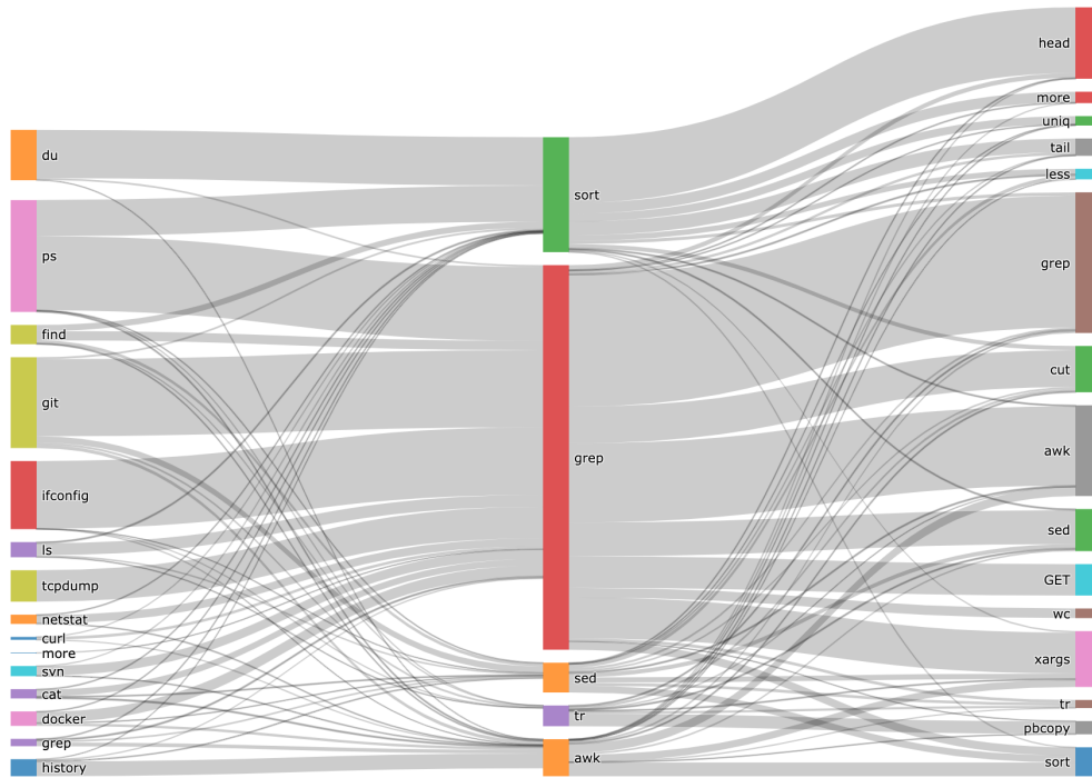
Figure 4: Flow diagram of the top 250 pipelines with three commands that make up at least 10 % of one command's usage
