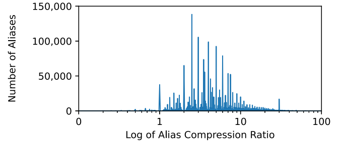
Figure 3: Distribution of alias compression ratios
