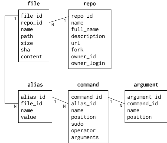
Figure 1: Relational database schema.
